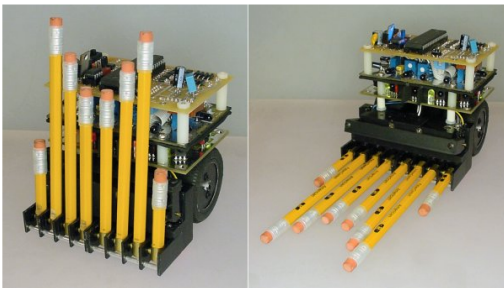
Front views of No.2, a champion autonomous mini-sumo robot
